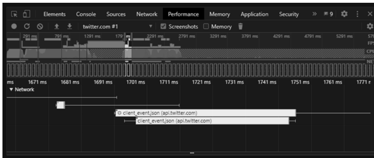
Figure 4-2: The DevTool's Performance tab showing the exact moment the Twitter application interacted with the Twitter API
