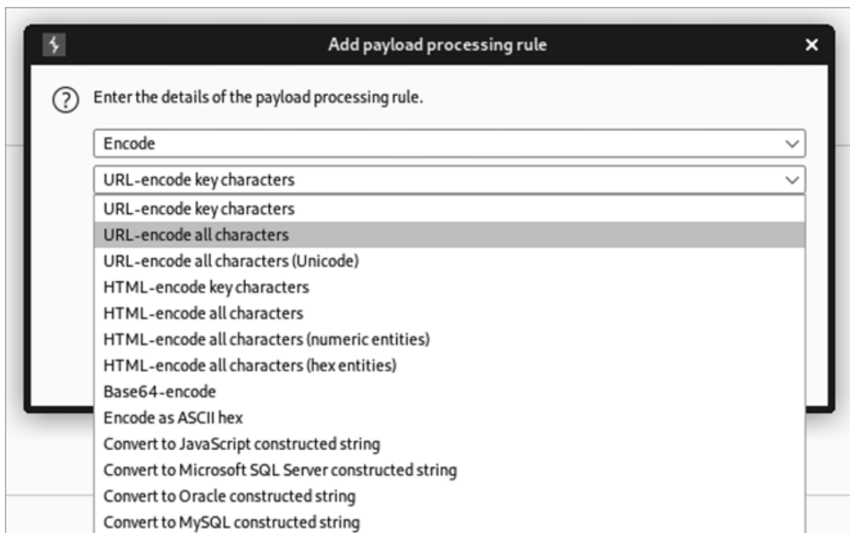
Figure 13-2: The Add Payload Processing Rule screen
