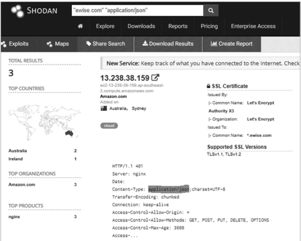
Figure 6-5: Shodan search results
