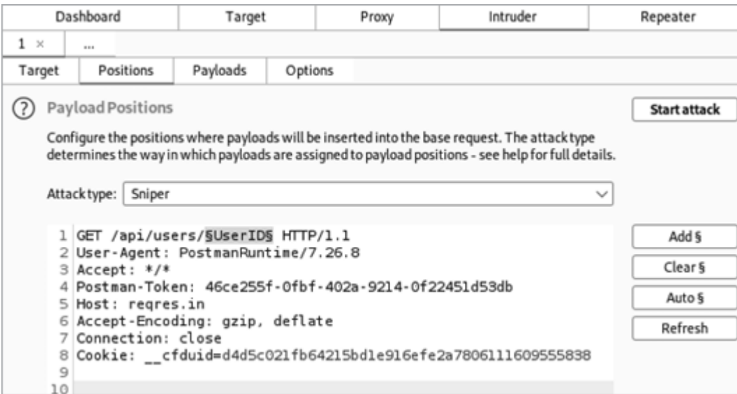
Figure 4-32: Burp Suite's Intruder configured with the attack position set around the UserID portion of the path
