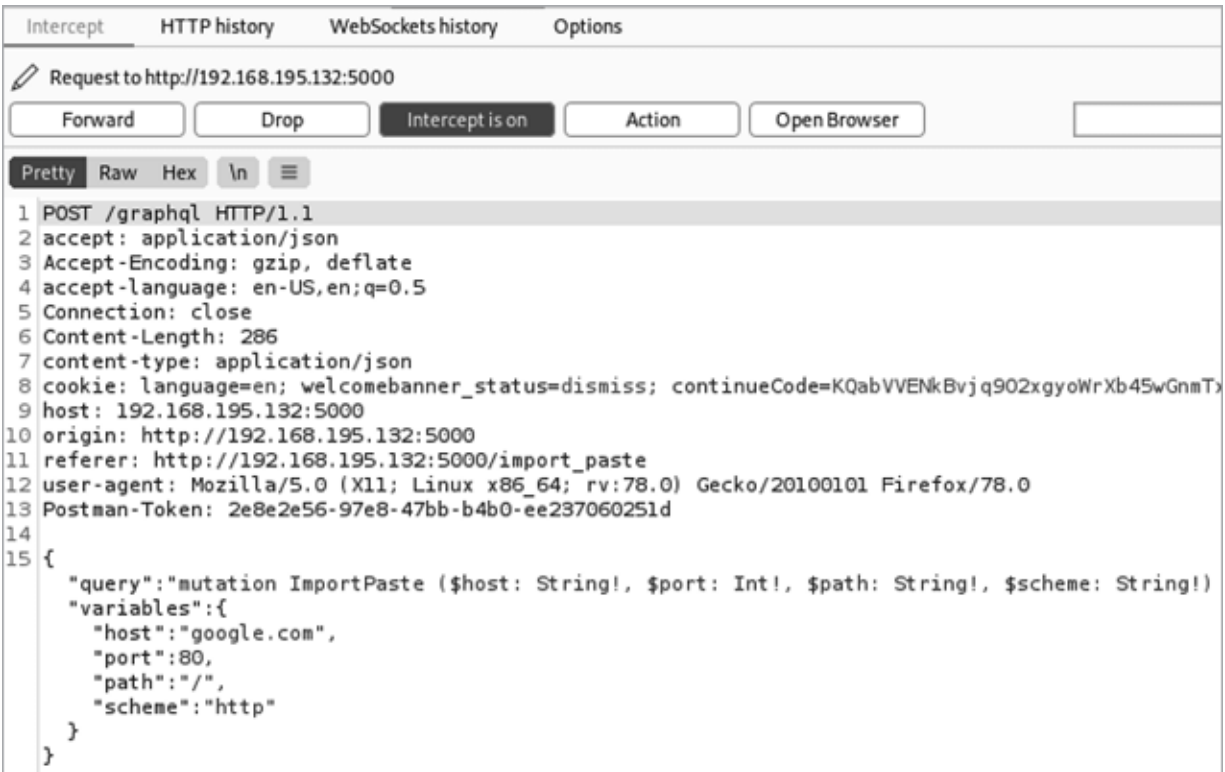
Figure 14-13: An intercepted GraphQL mutation request
