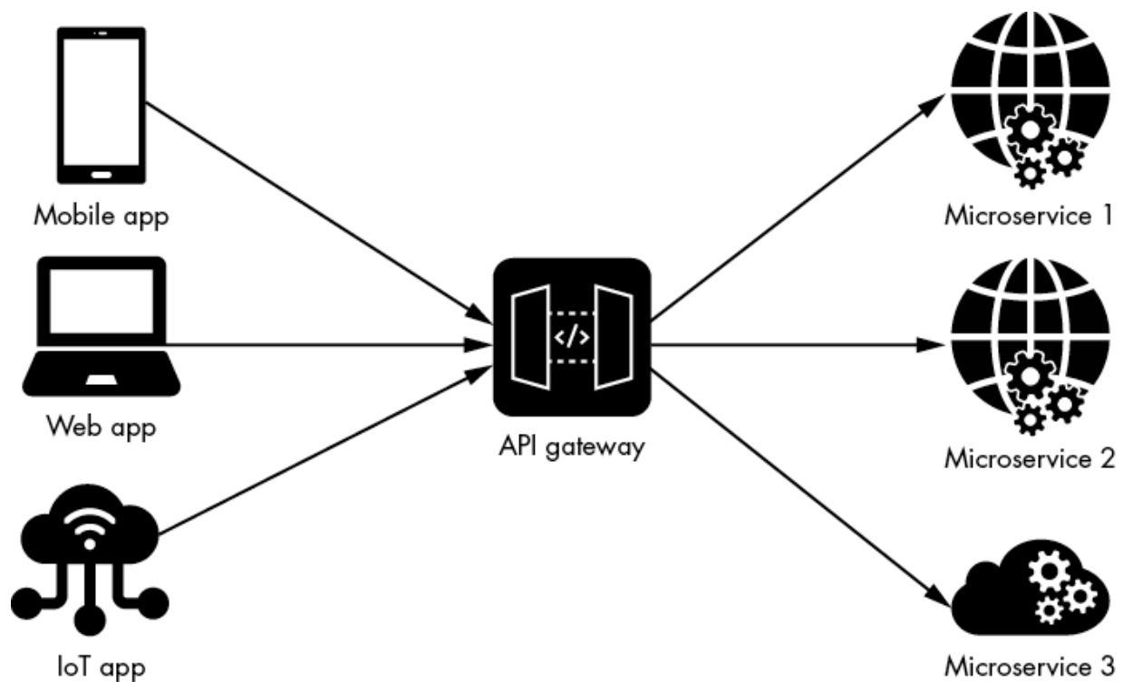
Figure 2-1: A sample microservices architecture and API gateway
