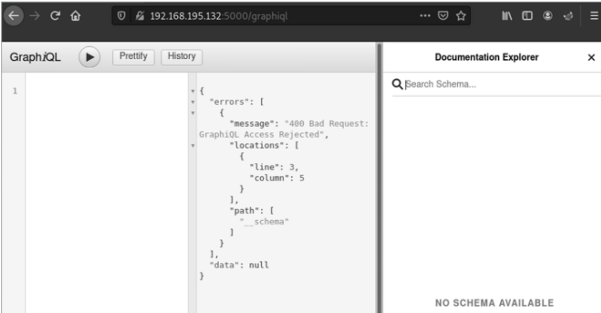
Figure 14-5: The DVGA GraphiQL web IDE
