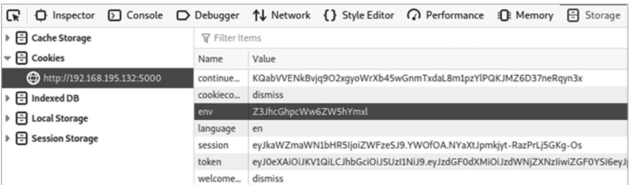
Figure 14-7: Cookies in DevTools
