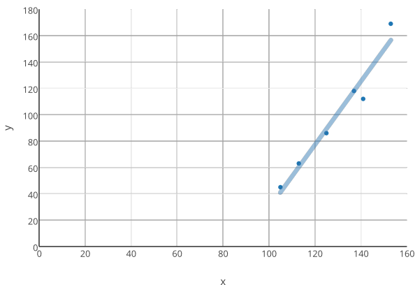
Figure 7.6: The affine model (y_{\vec{m}'}(x) = m_0 + m_1x) that best fits the data points is the line y(x) = -210.4 + 2.397x . Allowing for one extra parameter, m_0 (the y -intercept), results in a model that fits the data much better, as compared to the fit in Figure 7.4.
