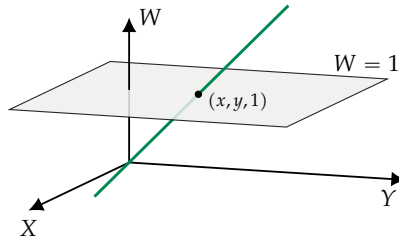
Figure 7.7: A two-dimensional Cartesian point (x, y)_c corresponds to an infinite line in a three-dimensional homogeneous coordinates space \{(\alpha x, \alpha y, \alpha)_h, \alpha \in \mathbb{R}\} . To convert a point from homogeneous coordinates to Cartesian coordinates, we must find where the infinite line intersects the plane W = 1 . The homogeneous coordinates of the intersection point will have the form (x, y, 1)_h . The first two components of this point are the Cartesian coordinates (x, y)_c .
