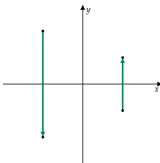
Figure 5.7: The reflection through the x -axis sends every point (x, y) in the plane to its mirror point (x, -y) on the other side of the x -axis.
