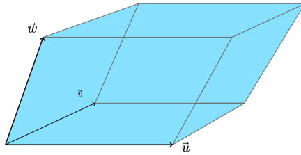
Figure 3.9: The determinant of a 3 \times 3 matrix corresponds to the volume of the parallelepiped constructed from the rows of the matrix.
