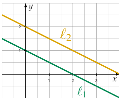
Figure 1.68: Case B: The lines with equations x + 2y = 2 and x + 2y = 4 are parallel and do not intersect. Using set notation, we can describe the solution set as \emptyset (the empty set).
