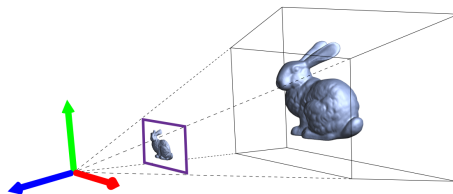
Figure 7.13: The perspective transformation that projects a three-dimensional model onto a two-dimensional screen surface. Note only a subset of the scene (the view frustum ) is drawn, which lies between the near plane and the far plane within the field of view.
