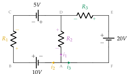
Figure 7.2: The circuit with branch currents labelled. Each resistor is assigned a polarity relative to the current flowing through it.
