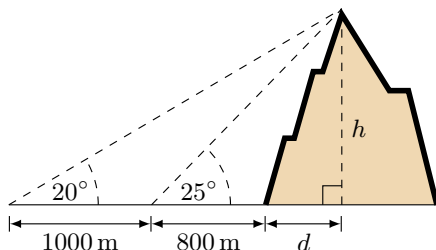
Figure 1.70: Measuring the height of a mountain using angles.
