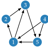
Figure 7.3: A simple graph with five vertices and seven edges.
