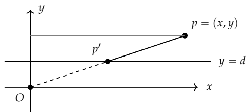
Figure 7.10: The point p' = (x', y') is the projection of the point p = (x, y) onto the line with equation y = d . The ratio of lengths d/y must equal the ratio of lengths x'/x .
