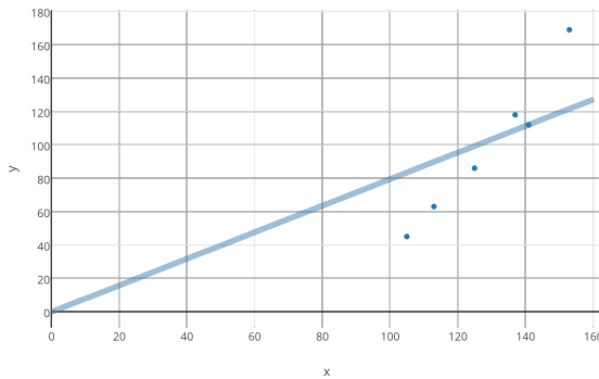
Figure 7.4: The line of the form y_m(x) = mx that best fits the set of data points (x_i, b_i) \in \mathbb{R}^2 . The plot shows a scatter plot of the data points, and the line of best fit y(x) = 0.792x . The line passes through the middle of the dataset and minimizes the sum of the squared vertical differences between the model output y_m(x_i) and the true value b_i .
