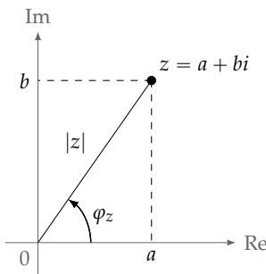
Figure 1.57: The complex number z = a + bi corresponds to the point with coordinates (a, b) in the complex plane.
