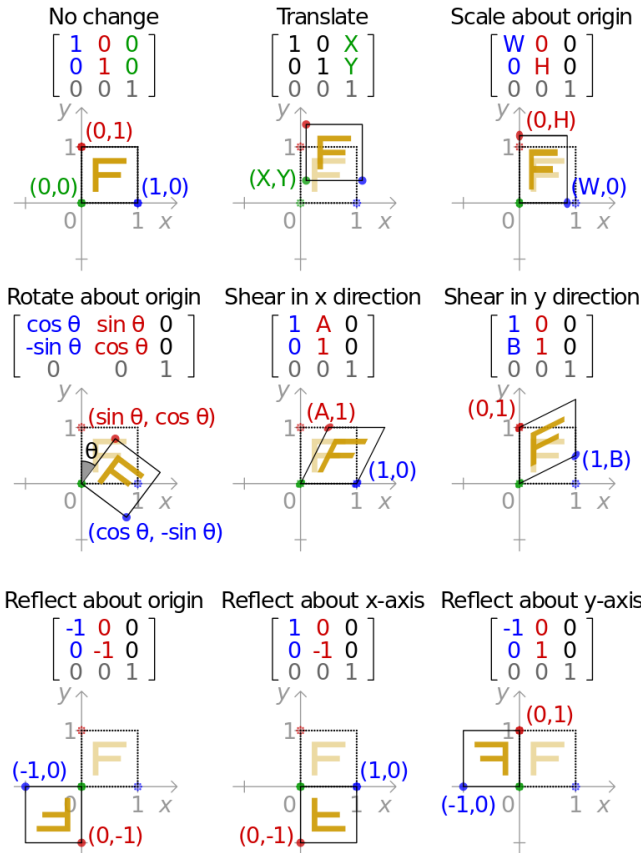
Figure 7.8: Illustration of the different transformations on a sample shape. Source: wikipedia File:2D_affine_transformation_matrix.svg
