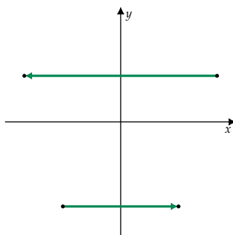
Figure 5.8: The reflection through the y -axis flips the x -component of every point in the plane.
