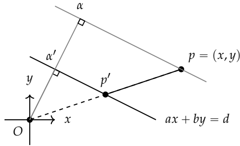
Figure 7.11: The point p' = (x', y') is the projection of the point p = (x, y) onto the line with equation ax + by = d . We define points \alpha' and \alpha in the direction of line's normal vector \vec{n} = (a, b) . The distances from the origin to these points are \ell' and \ell respectively. We have \ell'/\ell = x'/x = y'/y .
