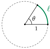
Figure 1.36: The angle \theta measured in radians corresponds to the arc length \ell on a circle with radius 1. The full circle corresponds to the angle 2\pi rad.
