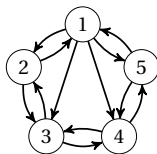
Figure 8.3: Graph showing five webpages and the links between them.
