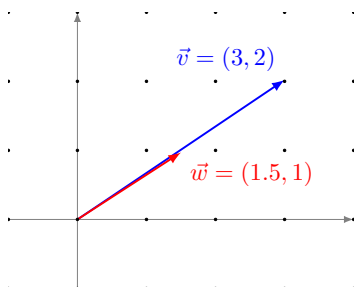
Figure 1.51: Vectors \vec{v} and \vec{w} are related by the equation \vec{v} = 2\vec{w} .
