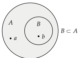
Figure 1.65: Venn diagram showing an example of the set relation B \subset A . The set B is strictly contained in the set A .
