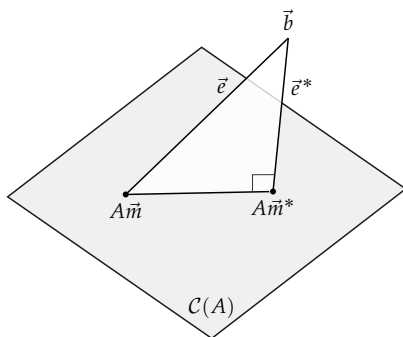
Figure 7.5: Linear regression can be seen as a “search” problem restricted to the column space of the data matrix A . The least squares approximate solution \vec{m}^* = A^+ \vec{b} corresponds to the point in \mathcal{C}(A) that is closest to \vec{b} . For this \vec{m}^* , the error vector \vec{e}^* is perpendicular to the column space of A .
