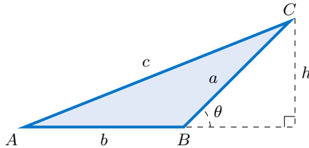
Figure 1.71: A triangle with base b and height h .
