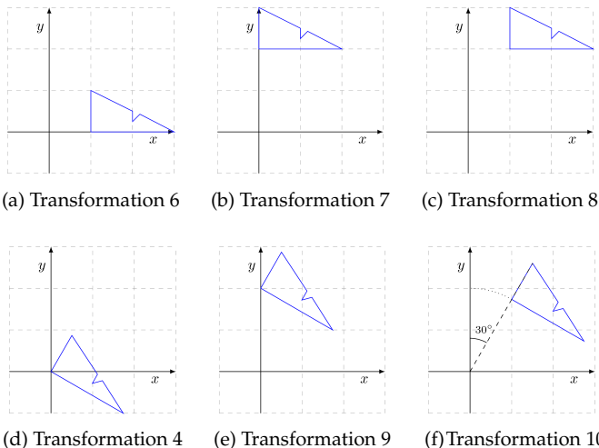
Figure 7.21: The effects of various affine transformations on the triangular shape shown in Figure 7.20 (a).
