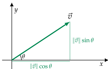
Figure 1.52: The x - and y -components of a vector with length \|\vec{v}\| in the direction \theta are given by v_x = \|\vec{v}\| \cos \theta and v_y = \|\vec{v}\| \sin \theta .
