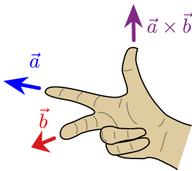
Figure 2.2: Using the right-hand rule to determine the direction of the cross product \vec{a} \times \vec{b} based on directions of \vec{a} and \vec{b} .
