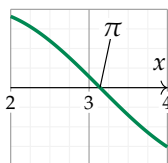
Figure 1.27: The function f(x) = \sin(x) crosses the x -axis at x = \pi .
