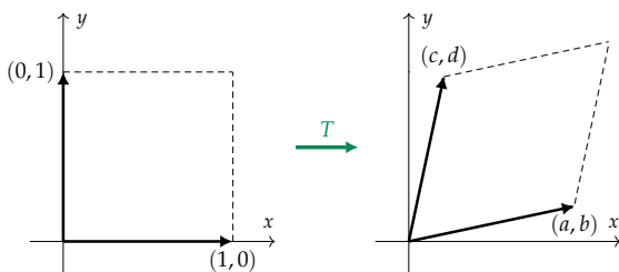
Figure 3.6: A square with side length 1 in the input space of T is transformed to a parallelogram with area \det(A_T) in the output space of T . The determinant measures the scale factor by which the area changes.
