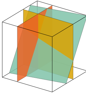
Figure 4.2: Three non-parallel planes in \mathbb{R}^3 intersect at a point.
