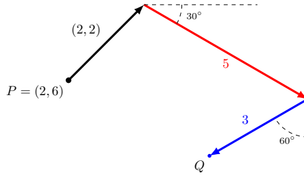
Figure 1.72: A point P is displaced by three vectors to obtain point Q .
