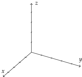
Figure 1.55: A three-dimensional coordinate system with x , y , and z axes.
