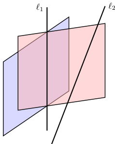
Figure 4.12: The line \ell_1 is the intersection of the two planes. In P4.9 we want to find the plane that contains \ell_1 and doesn't intersect \ell_2 .
