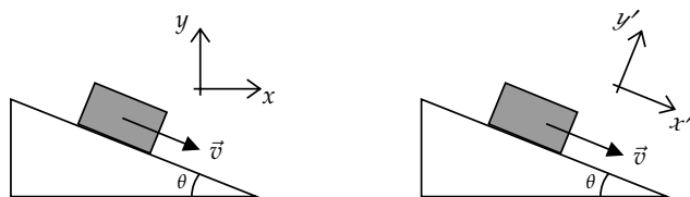
Figure 1.56: The vector \vec{v} is described by the coordinates (v \cos \theta, -v \sin \theta)_{xy} with respect to the standard basis xy . The same vector \vec{v} is described by the coordinates (v, 0)_{x'y'} with respect to the “tilted” basis x'y' .
