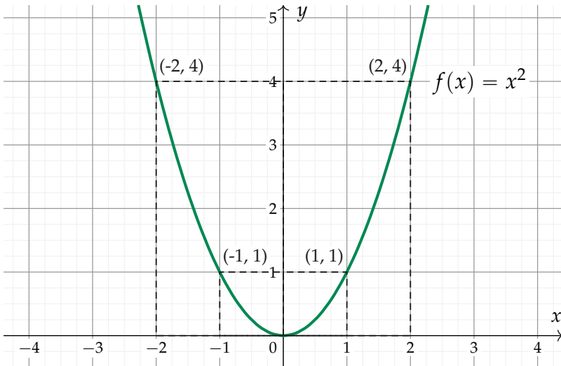
Figure 1.23: Plot of the quadratic function f(x) = x^2 . The graph of the function passes through the following (x,y) coordinates: (-2,4) , (-1,1) , (0,0) , (1,1) , (2,4) , (3,9) , etc.
