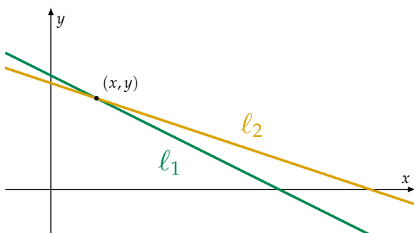
Figure 1.61: The point (x, y) that lies at the intersection of lines \ell_1 and \ell_2 .
