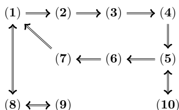
Figure 5.12: The chain of implications used to prove the invertible matrix theorem.
