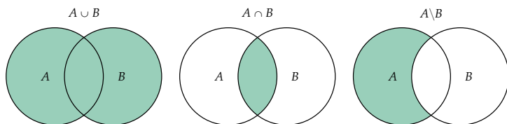
Figure 1.66: Venn diagrams showing different subsets obtained using the set operations: set union A \cup B , set intersection A \cap B , and set difference A \setminus B .
