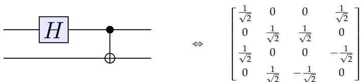
Figure 9.20: A quantum circuit that applies the Hadamard gate to the first qubit, then applies the controlled-NOT gate from the first qubit to the second qubit.
