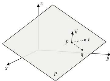
Figure 4.7: We can obtain the normal vector \vec{n} for the plane P by starting from the three points p , q , and r which lie in the plane.
