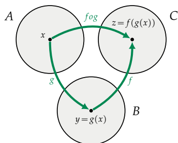
Figure 1.19: The function composition f \circ g describes the combination of first applying the function g , followed by the function f : f \circ g(x) = f(g(x)) .
