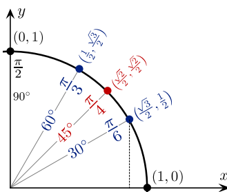
Figure 1.43: The combined (\cos \theta, \sin \theta) coordinates for the points on the unit circle at the most common angles: 0 , \frac{\pi}{6} ( 30^\circ ), \frac{\pi}{4} ( 45^\circ ), \frac{\pi}{3} ( 60^\circ ), and \frac{\pi}{2} ( 90^\circ ).
